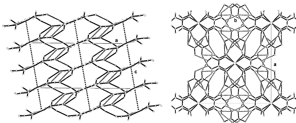
Figure 4. Views along the b (left) and c (right) crystallographic axes of the molecular packing of 4 . The selection criteria for hydrogen bonds (depicted as thin dotted lines) were: d(\text{N}\cdots\text{O}) < R(\text{N}) + R(\text{O}) + 0.50 , d(\text{H}\cdots\text{O}) < R(\text{H}) + R(\text{O}) - 0.12 , \text{N}-\text{H}\cdots\text{O} > 100.0^\circ .
