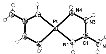
Figure 3. ORTEP plot (50% thermal probability ellipsoids) of the crystal structure of 4 ; nitrate counterions are omitted. Selected bond lengths [Å] and angles [°]: Pt–N1 1.996(6), Pt–N4 2.031(6), N1–C1 1.305(10), C1–N2 1.331(10), C1–N3 1.348(10), N4–N3 1.434(9), N1–Pt–N4 80.0(2), C1–N1–Pt 116.2(5), N1–C1–N2 125.8(8), N1–C1–N3 117.0(6), C1–N3–N4 116.6(5), N3–N4–Pt 110.1(4), N2–C1–N3 116.8(7).
