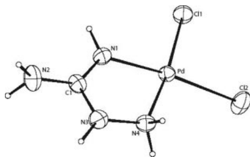
Figure 6. CAMERON plot (50% thermal probability ellipsoids) of the crystal structure of 6 ; selected bond lengths [Å] and angles [°]: Pd–Cl1 2.303(2), Pd–Cl2 2.322(2), Pd–N1 1.968(6), Pd–N4 2.019(5), C1–N1 1.307(8), C1–N2 1.339(9), C1–N3 1.347(9), N3–N4 1.407(8), Cl1–Pd–Cl2 93.86(6), Cl1–Pd–N1 92.7(2), Cl2–Pd–N4 92.5(2), N1–Pd–N4 81.0(2), N1–C1–N2 123.7(7), N1–C1–N3 117.9(6), N3–C1–N2 118.3(6).
