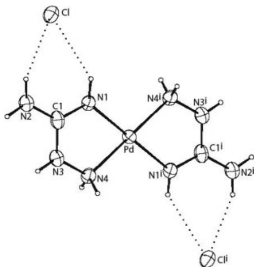
Figure 7. CAMERON plot (50% thermal probability ellipsoids) of the crystal structure of 7 . Selected bond lengths [Å] and angles [°]: Pd–N1 1.977(7), Pd–N4 2.029(7), C1–N1 1.303(11), C1–N2 1.341(12), C1–N3 1.358(11), N3–N4 1.401(9), H1...Cl 3.436(8), H21...Cl 3.288(9), N1–Pd–N4 80.6(3), Pd–N1–C1 115.2(6), N1–C1–N3 117.2(8), N2–C1–N3 116.8(9), N1–C1–N2 125.9(9), C1–N3–N4 116.9(7), N3–N4–Pd 109.7(5), N1–H1...Cl 142, N2–H21...Cl 151.
